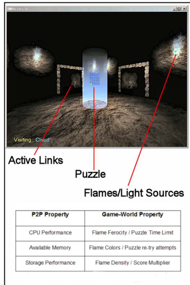
Figure 2: Modeling P2P Properties
