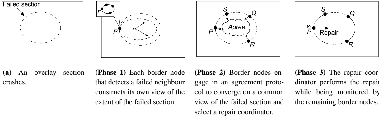
Figure 3. The three main phases of our repair algorithm
