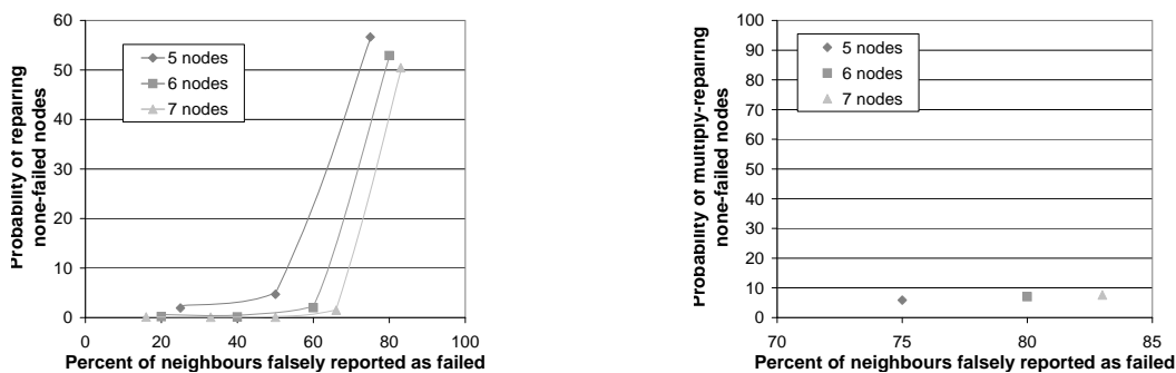
(a) Case 1: probabilities of repairing non-failed nodes, with increasing percentages of false positives and increasing mesh size
