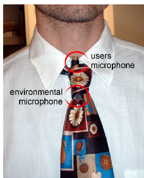
Figure 1: Context-Awareness Tie.
