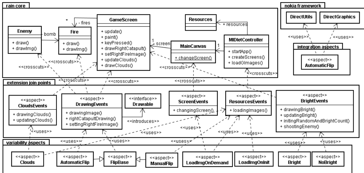
Figure 5. Architecture of the J2ME Game Product Line.
